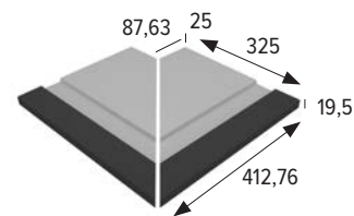
Angolo DX nicchia B33 SPORT Angle niche B33 SPORT
