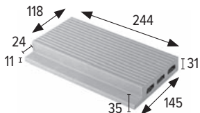
Supporto griglia Support de grille
